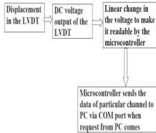
Fig.4 A Circuit Diagram of the Design architecture
