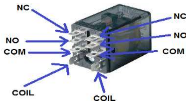
Fig.2 12v Relay DODT
