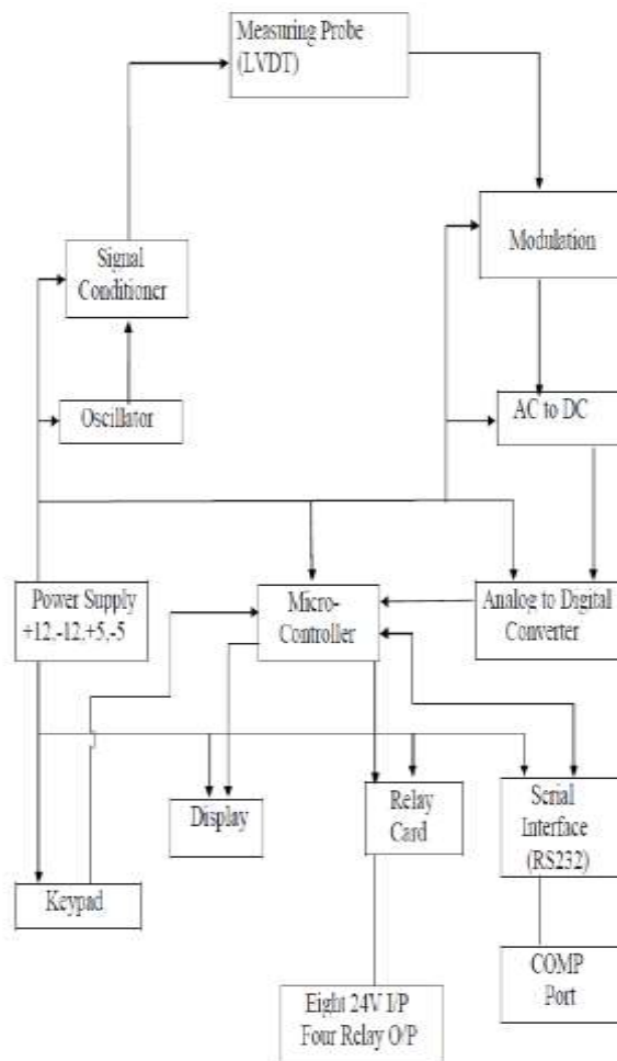
Fig.1 Block Diagram of Measuring Electronic Gauging System
